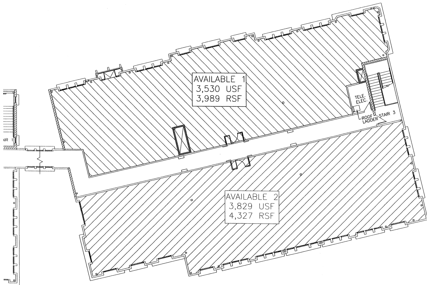
THIRD FLOOR TENANT PLAN SCALE: NTS
